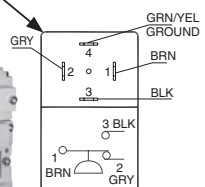
Status Indicator Cable with DIN Connector
