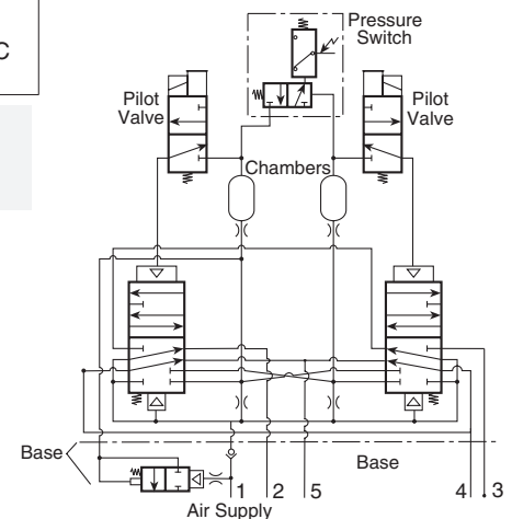
5/2 CrossMIRROR® double valve with pressure switch
