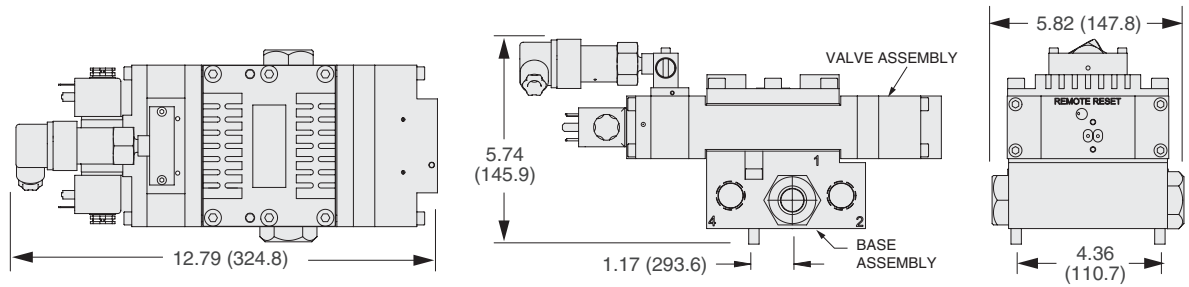
Basic Size 2 - Valve and base assembly, with remote reset and with pressure switch.
