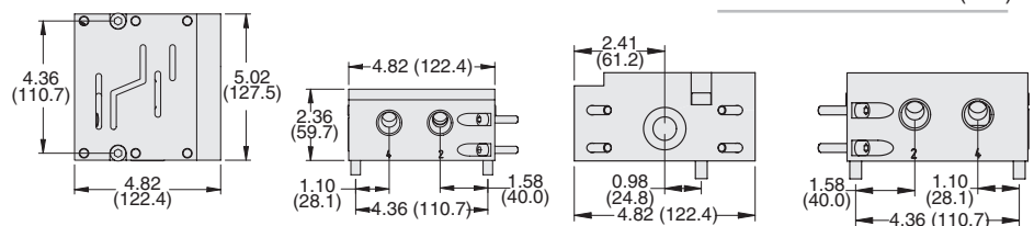
End Station for Basic Size 2
