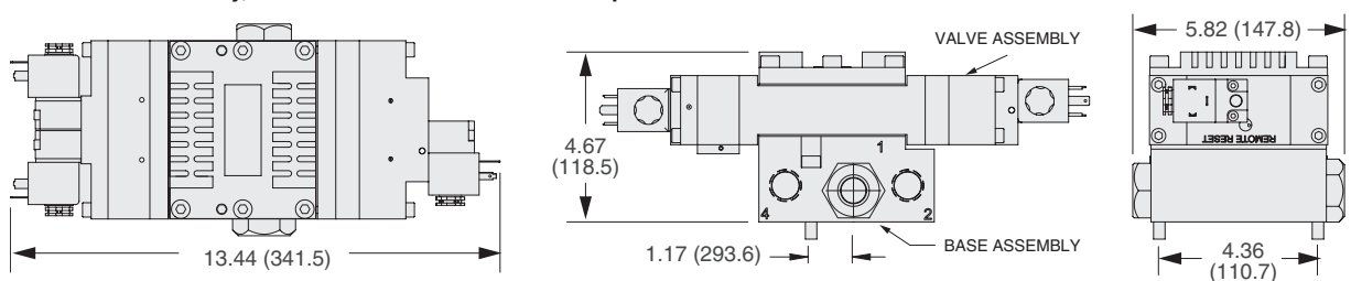
Basic Size 2 - Valve and base assembly, with solenoid reset and without pressure switch.
