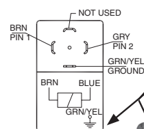
Solenoid Cables with M12 Connector
