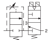
Simplified Schematic
